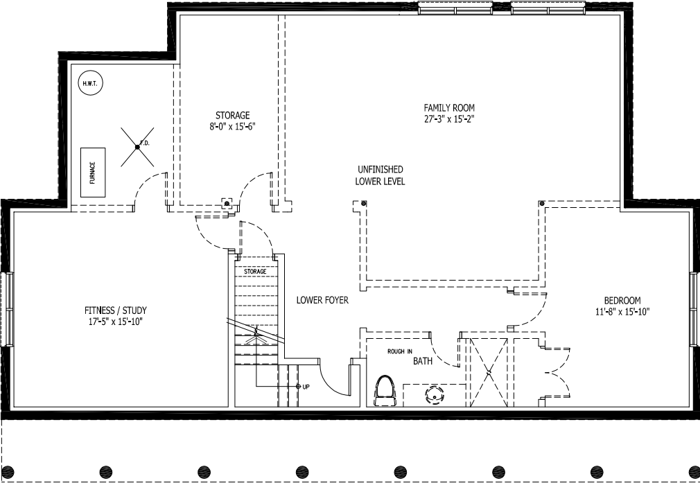
LOWER LEVEL 1,400 sq. ft.
