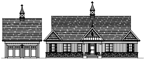
ELEV. B | without finished coach house
