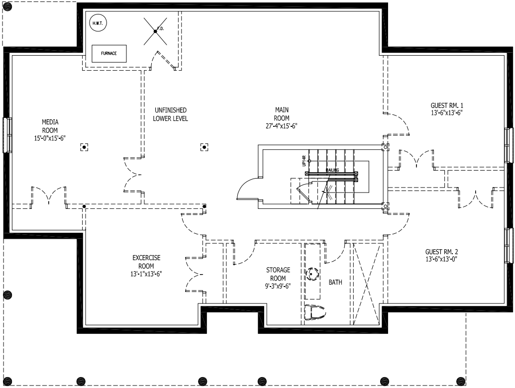
LOWER LEVEL 1,674 sq. ft. (34 sq. ft. finished lower foyer)
