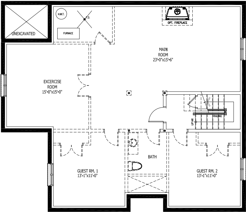
LOWER LEVEL 1,248 sq. ft. (34 sq. ft. finished lower foyer)
