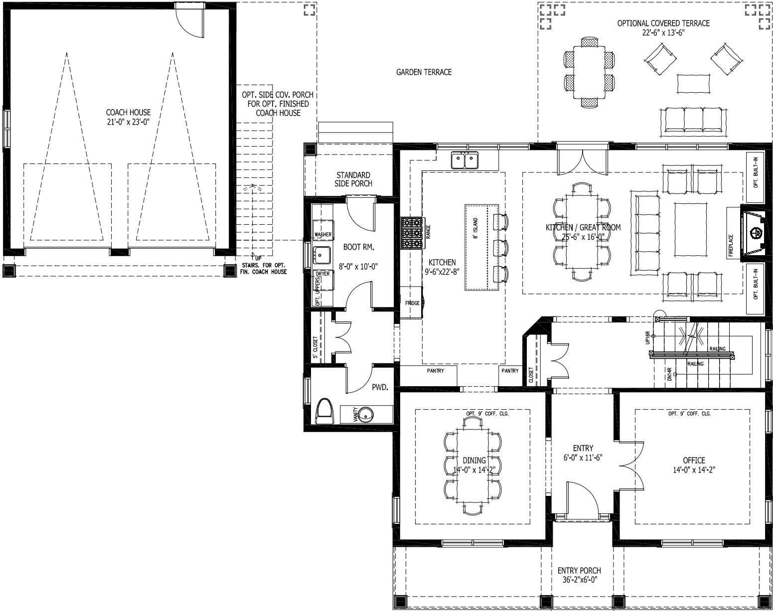
MAIN LEVEL 1,590 sq. ft.
