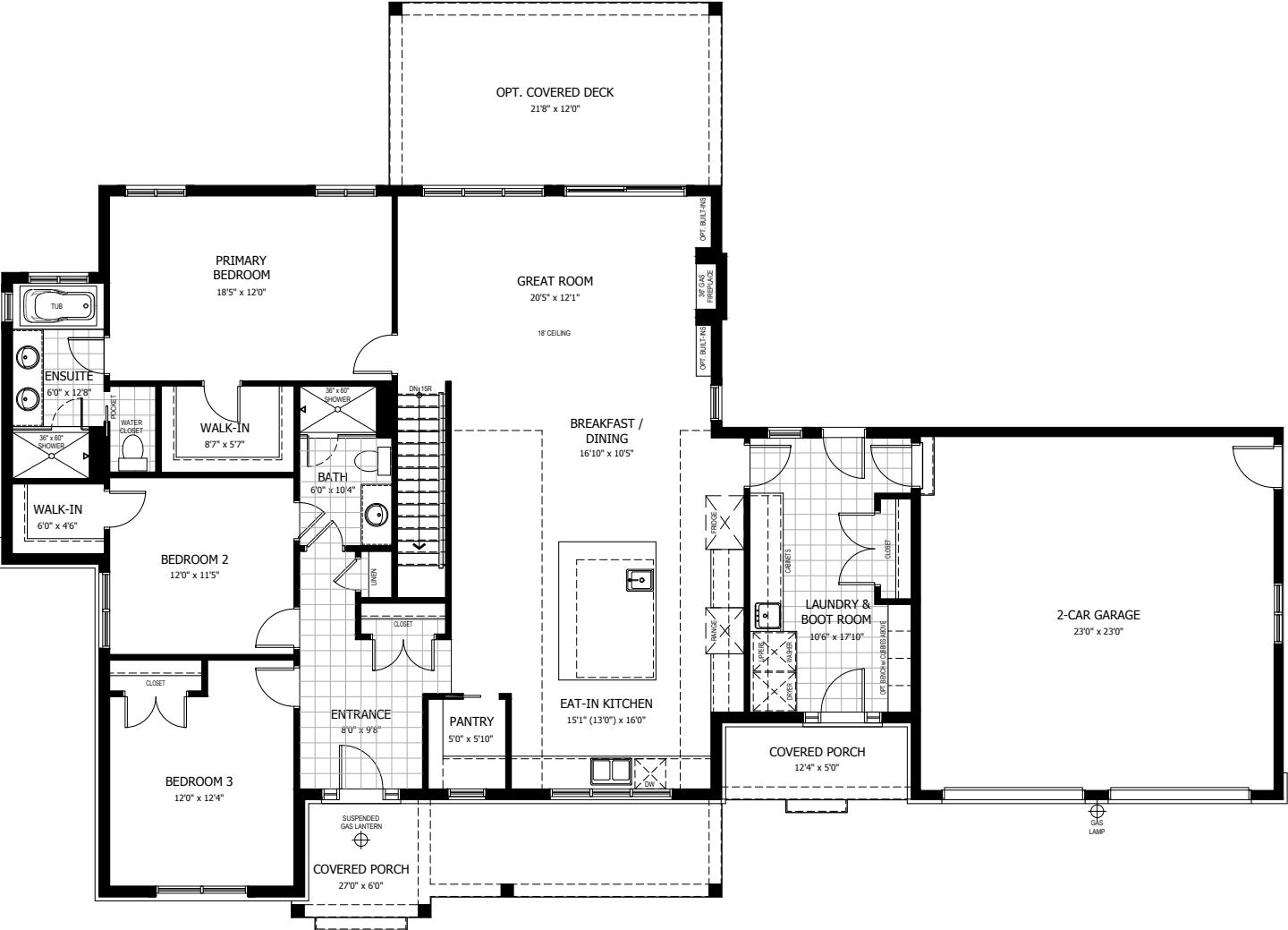
MAIN LEVEL 2,093 sq. ft.
