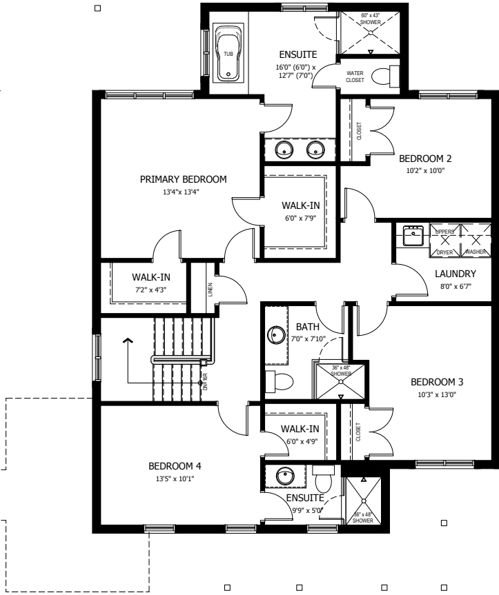
OPTIONAL UPPER FLOOR PLAN 1,334 sq. ft.
