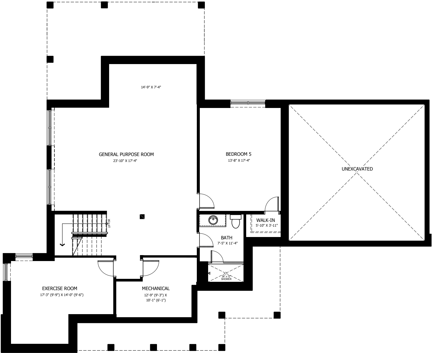
LOWER LEVEL OPTIONAL FINISHED 1,244 sq. ft.
