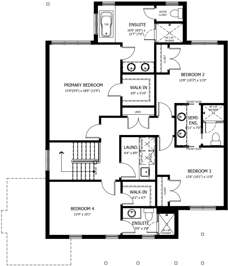
UPPER FLOOR PLAN 1,334 sq. ft.
