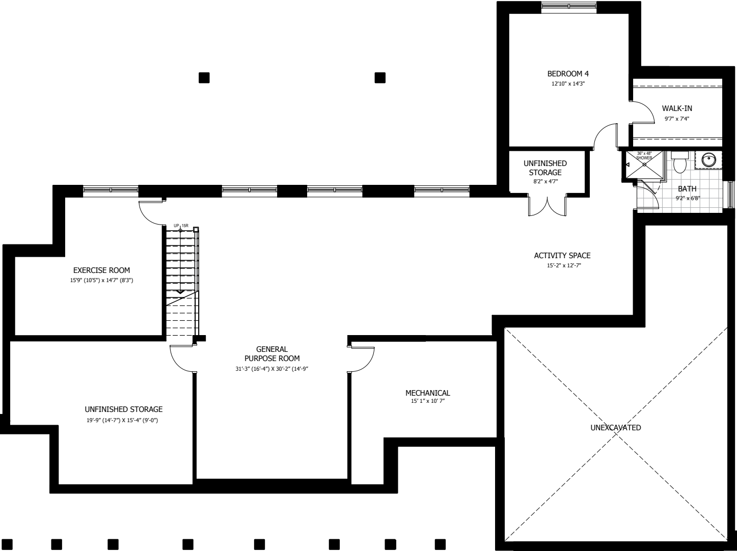
LOWER LEVEL OPTIONAL FINISHED 1,496 sq. ft.
