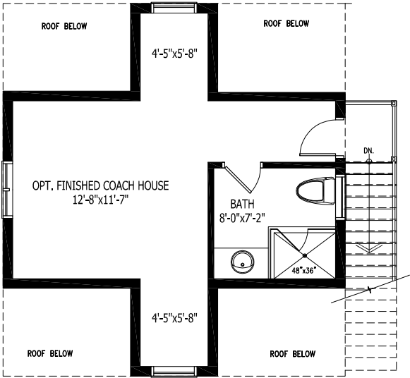
OPTIONAL FINISHED COACH HOUSE | ELEVATION A 350 sq. ft.
