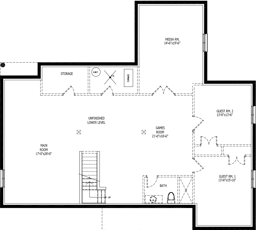
LOWER LEVEL 1,736 sq. ft.
