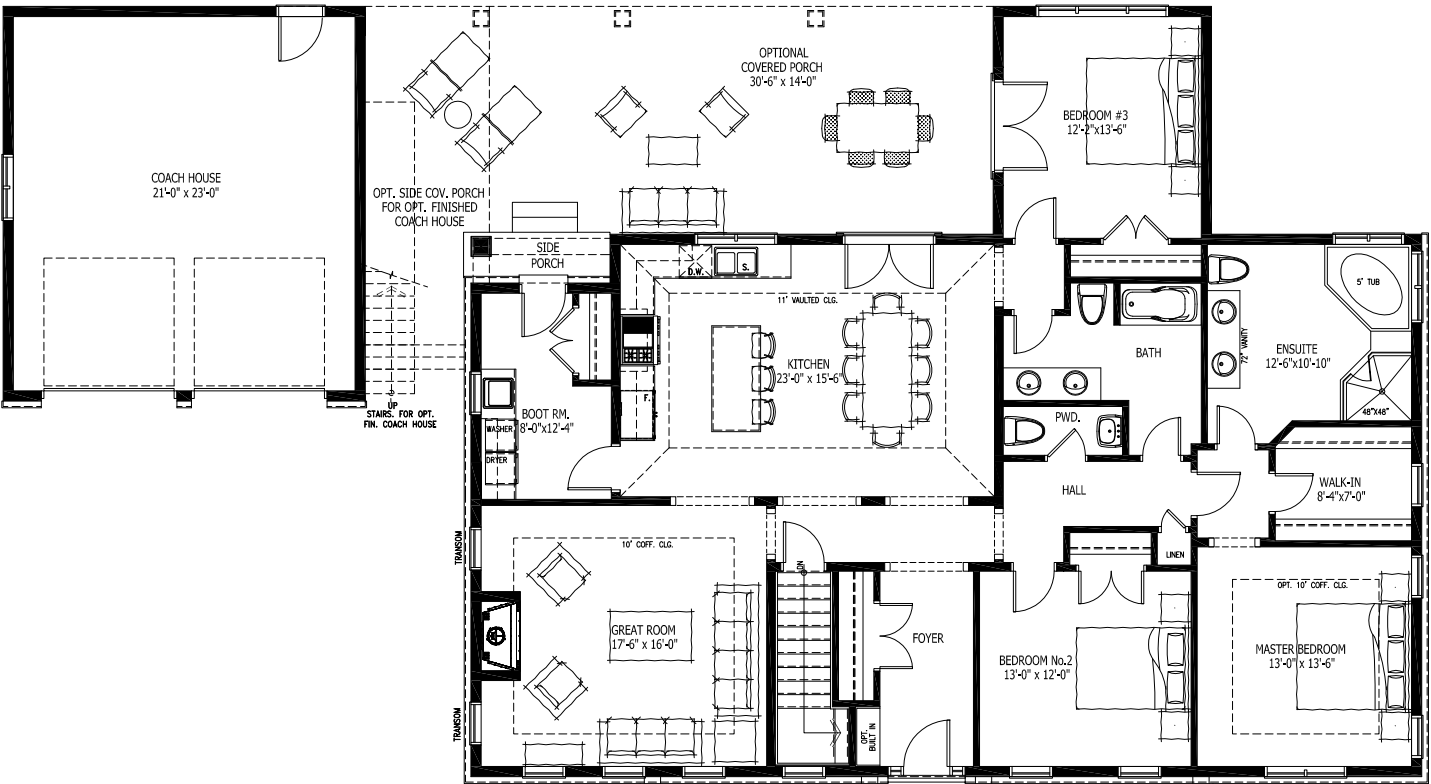
MAIN LEVEL 2,109 sq. ft.
